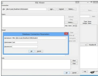
Figure 3: Connection with MySQL database using JDBC
