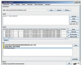
Figure 5: Database imported to WEKA
