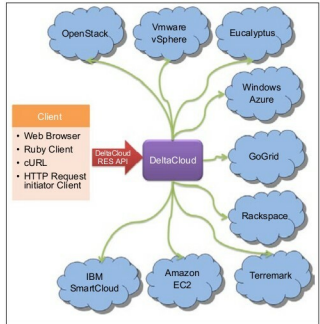
Figure 2: The Deltacloud API - How it works
