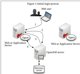
Figure 1: SSO-Initial Login process
