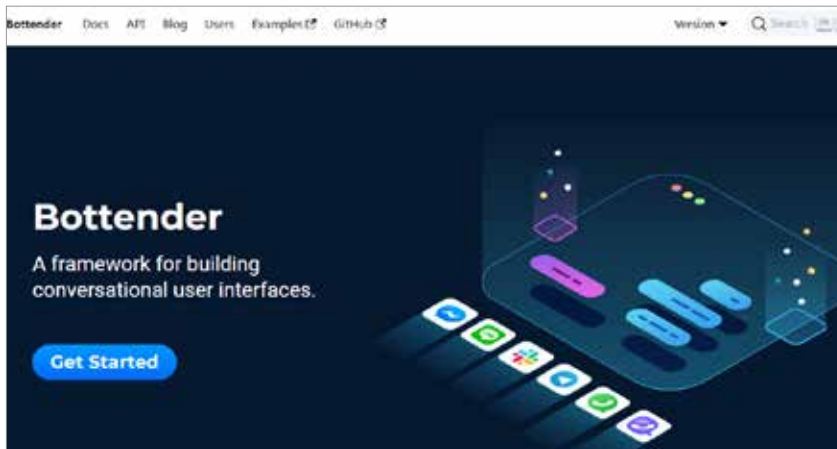
Figure 3: Bottender framework
