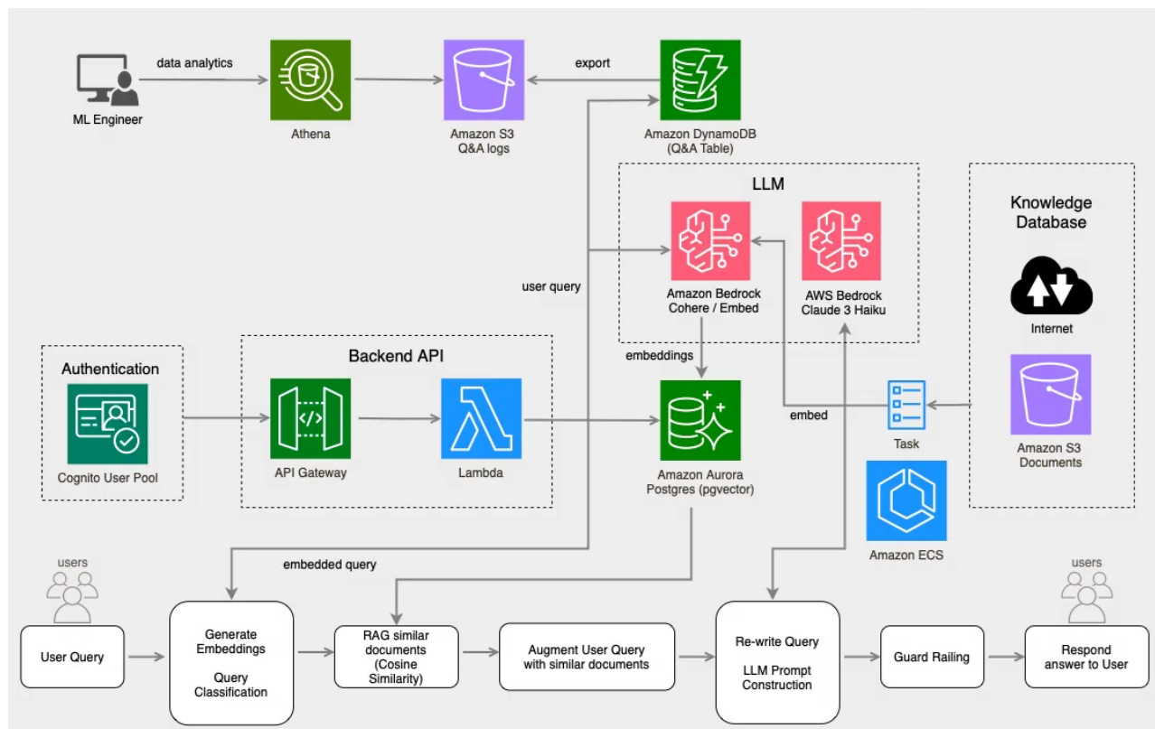
Figure 1: Reference architecture for Amazon Bedrock gen AI solution
