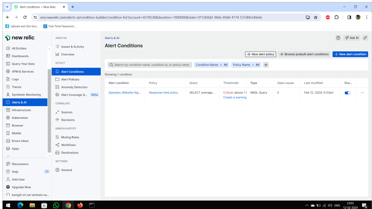
Figure 5: Sample alert to monitor the application
