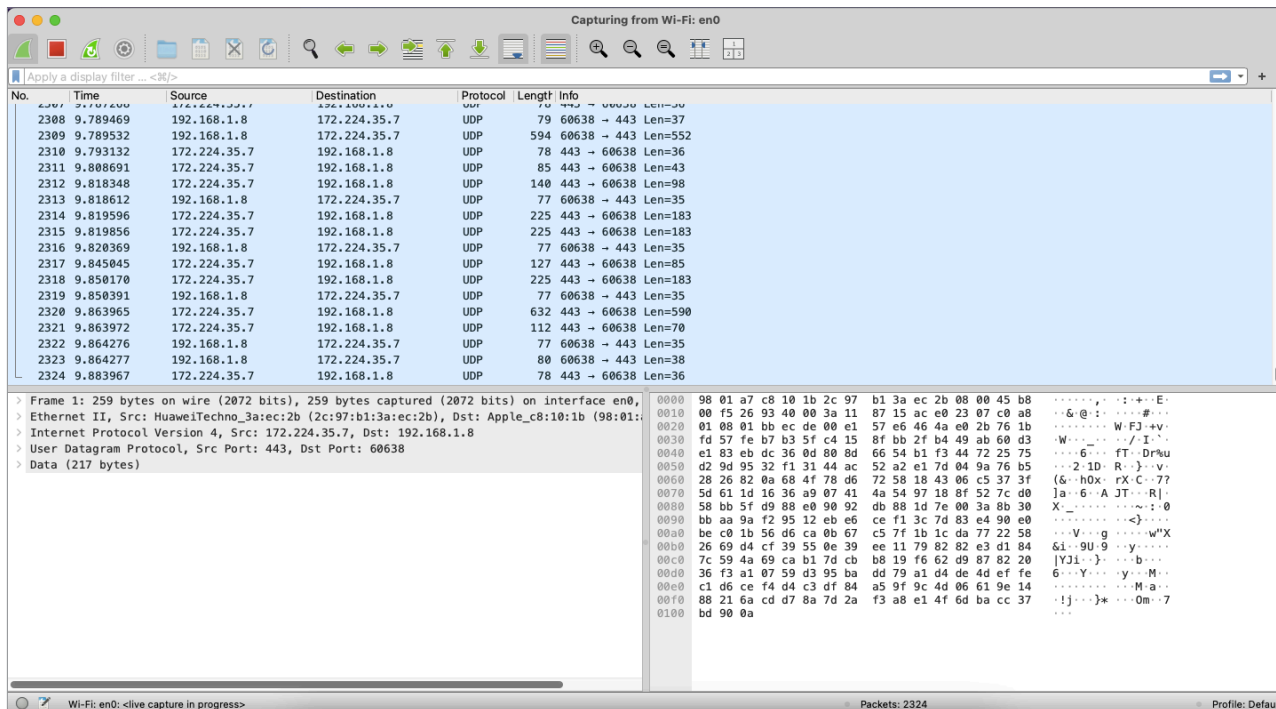
Figure 5: Packets on Wi-Fi
