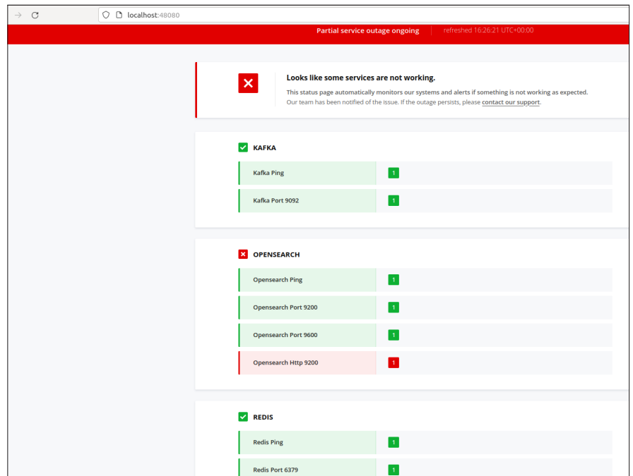
Figure 6: Vigil status page for multiple services probes
