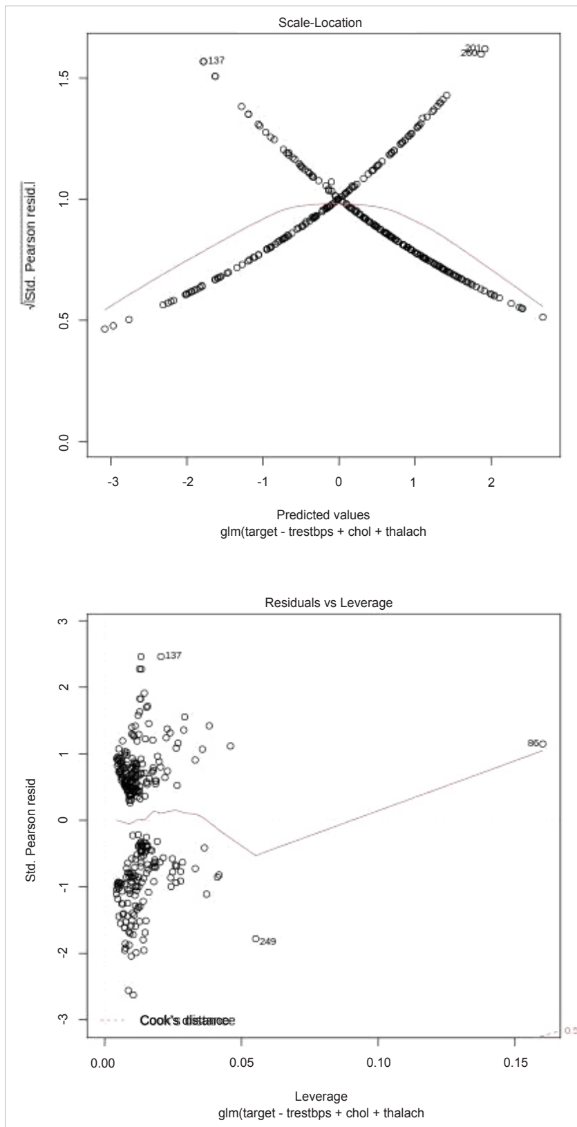
Figure 8: Graphical representation of residuals vs leverage
