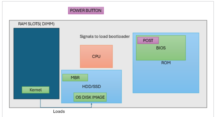
Figure 6: The kernel loading the operating system
