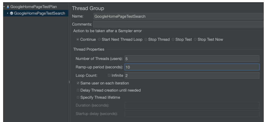
Figure 3: Thread group creation page
