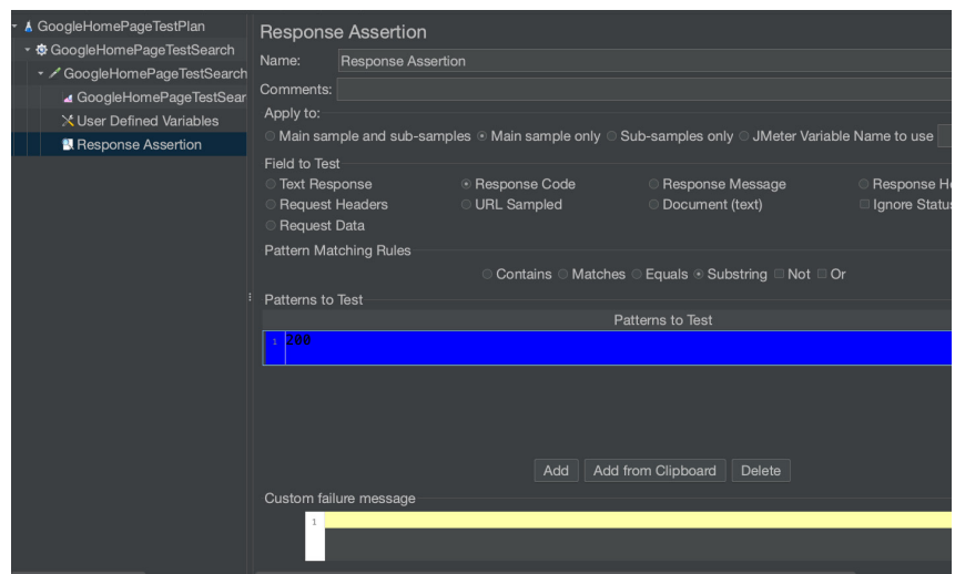
Figure 9: Define the rules to evaluate the response from the sampler execution
