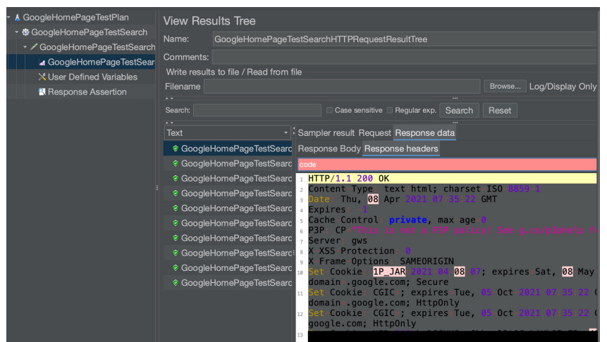
Figure 10: Response is 200; hence the test result is shown as passed (green)
