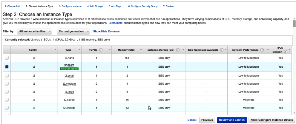
Figure 5: Select instance version
