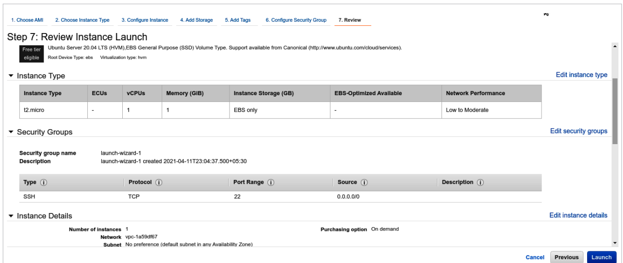
Figure 6: Launch instance
