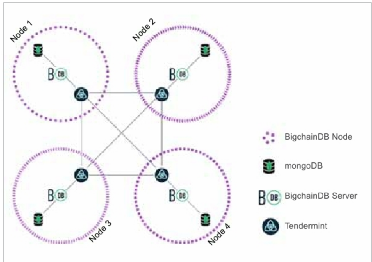
Figure 1: The four main components in the BigchainDB network
