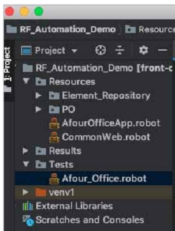
Figure 6: Project structure
