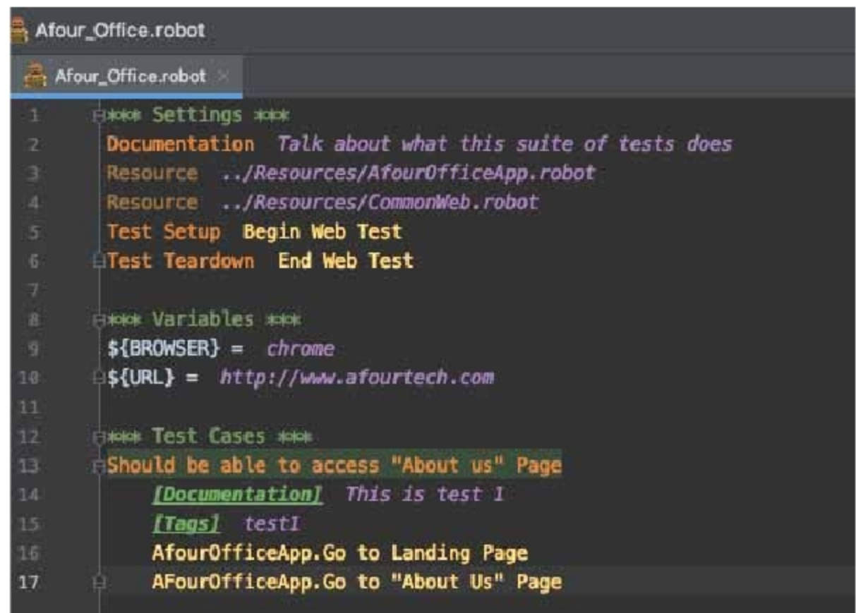
Figure 7: Test script
