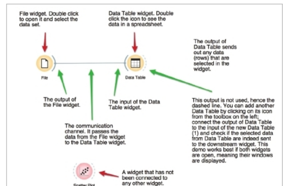
Figure 4: Data exploration
