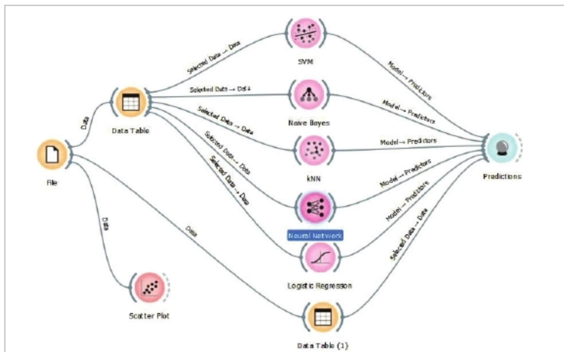
Figure 11: Applying different machine learning classifiers on the iris data set using Orange
