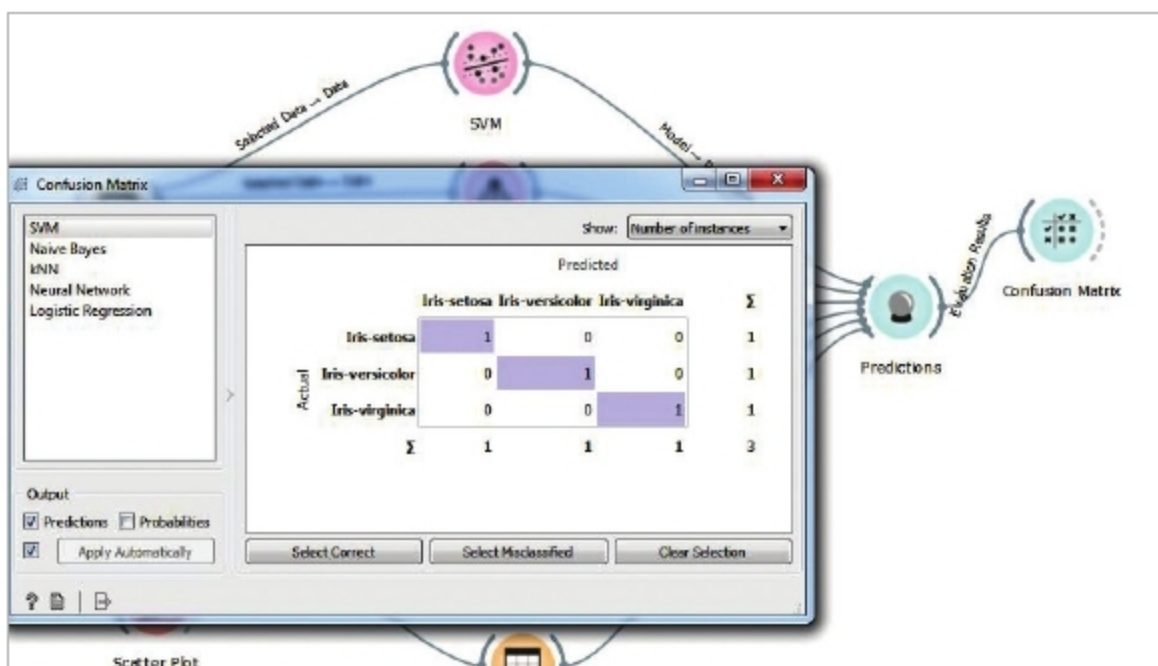
Figure 13: Confusion matrix for different machine learning classifiers – a performance analysis
