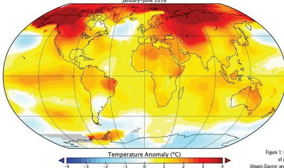
Global Mean Surface Temperature (GISS) January-June 2016
