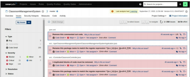
Figure 9: List of bugs in the code according to severity
