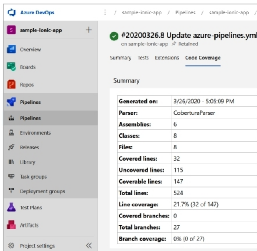
Figure 7: Code coverage report in the Azure DevOps portal
