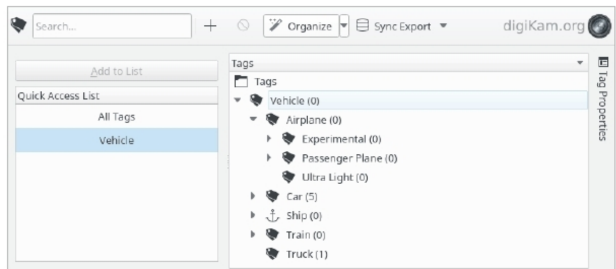
Figure 2: Tag manager
