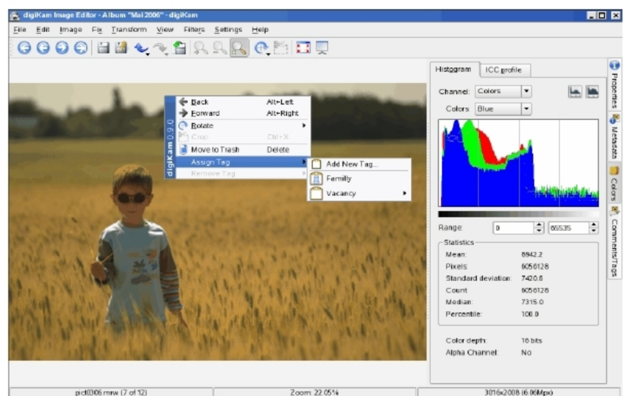
Figure 3: Image editor
