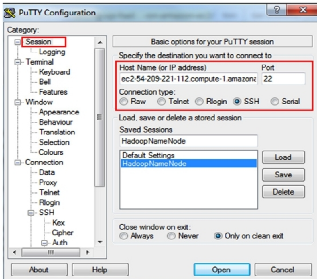
Figure 4: Choose Open to start the PuTTY session
