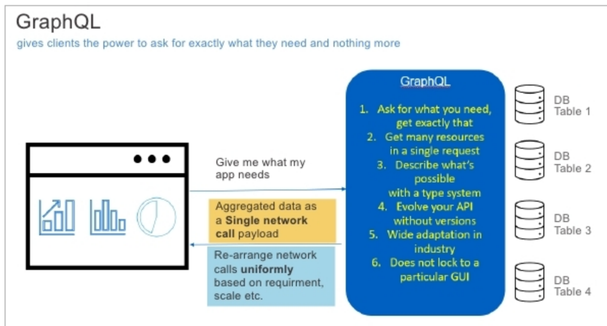
Figure 2: A helicopter view of GraphQL
