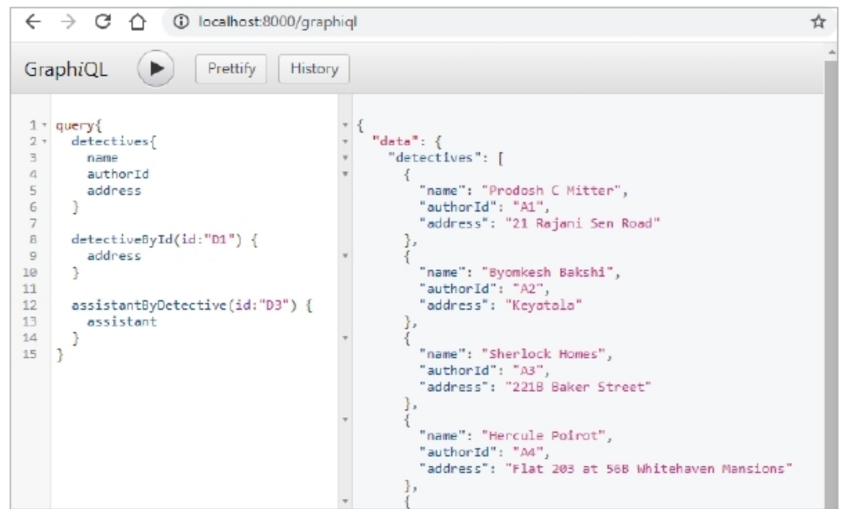
Figure 4: GraphQL app running queries
