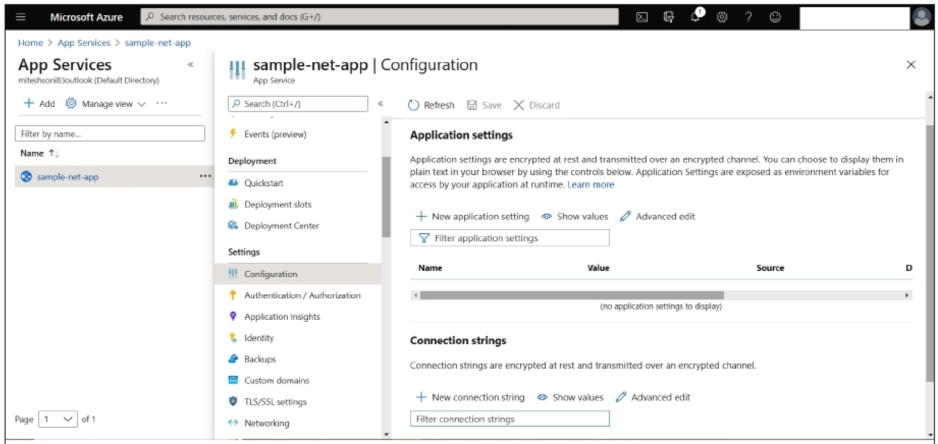
Figure 6: App Service: Configuration -- app settings
