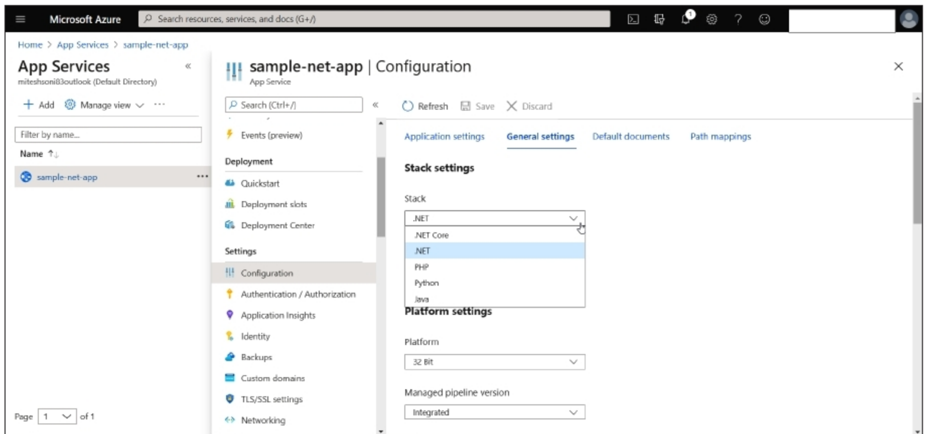
Figure 7: App Service: General settings
