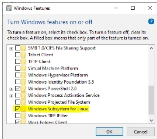
Figure 1: Enable WSL
