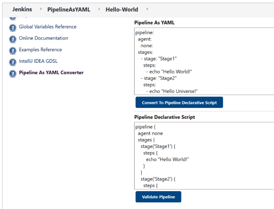
Figure 9: Valid pipeline declarative script
