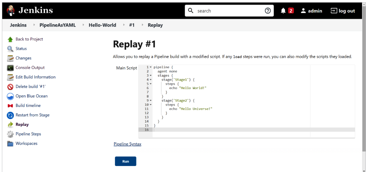
Figure 8: Replay pipeline
