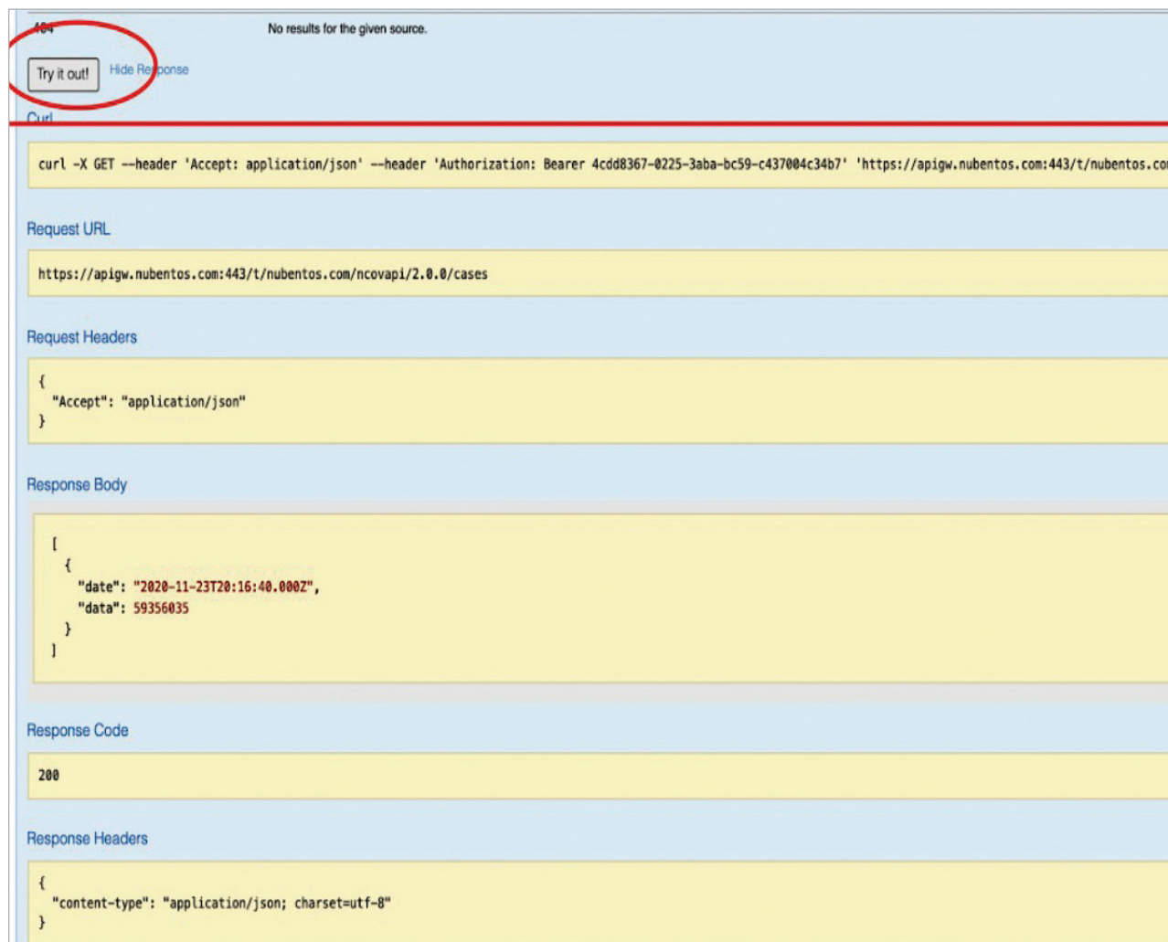
Figure 9: API-nCov19: Try out the endpoint to understand request/response json data format
