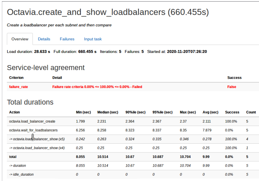
Figure 5: Result of Octavia.create_and_show_loadbalancers task using Amphora
