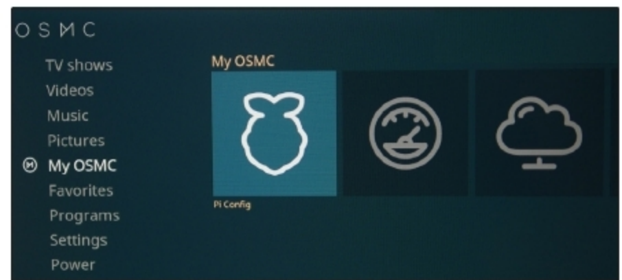
Figure 7: OSMC GUI
