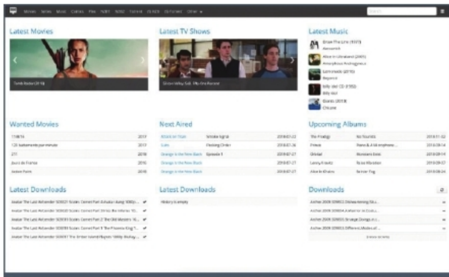
Figure 6: OpenFLIXR GUI
