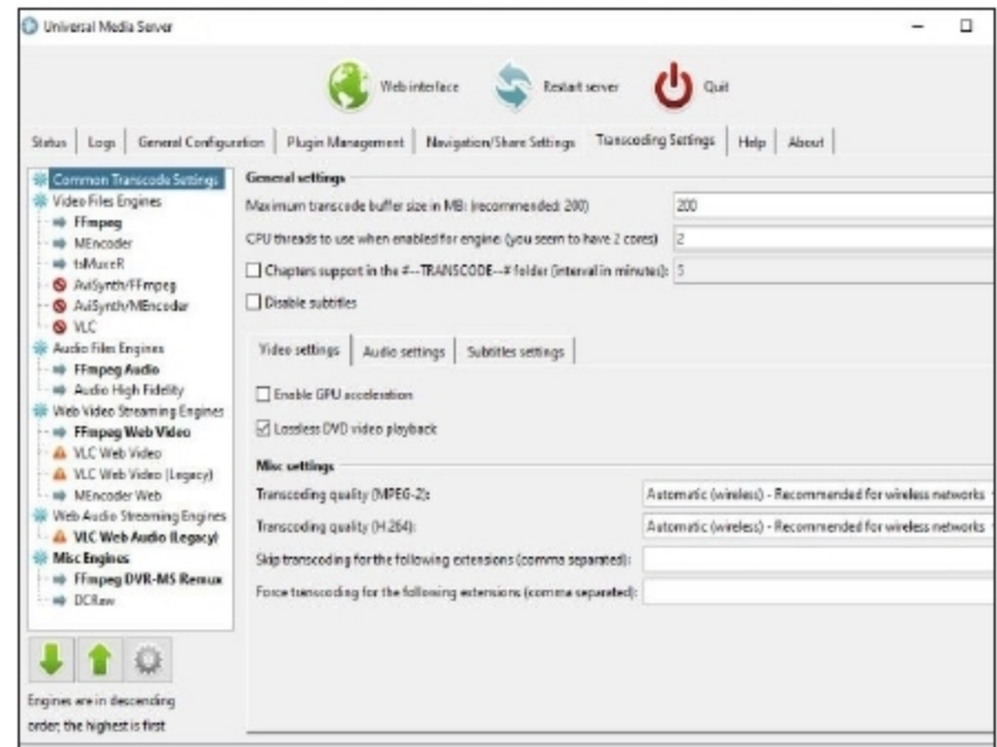
Figure 10: Universal Media Server (UMS) GUI
