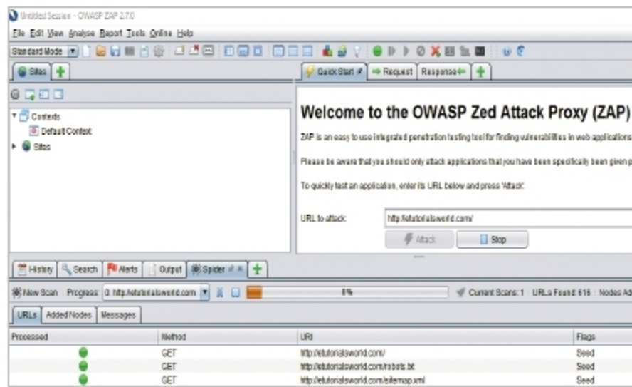
Figure 8: ZAP dashboard
