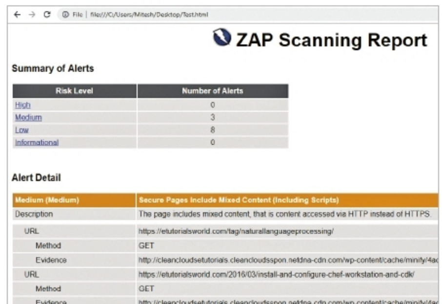
Figure 9: ZAP HTML report
