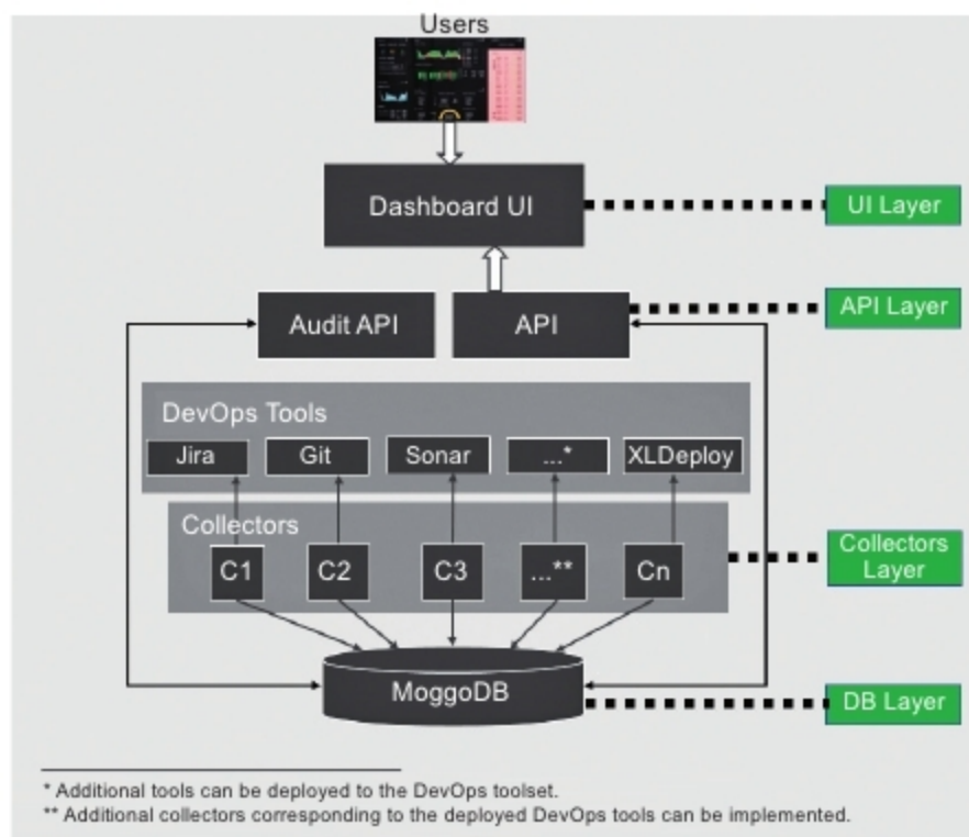
Figure 1: Architecture of Hygieia
