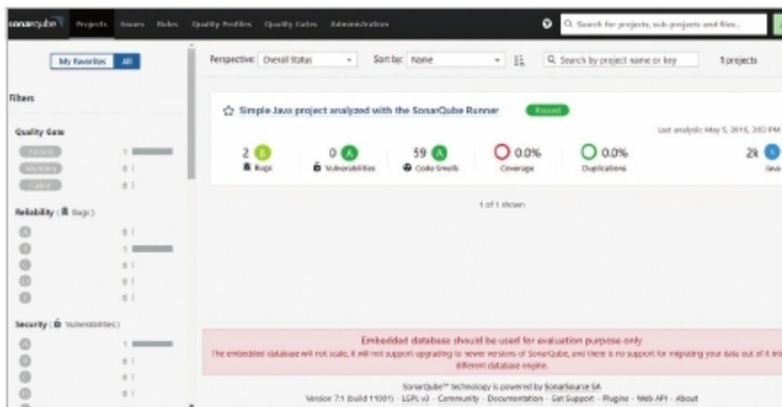
Figure 2: SonarQube dashboard
