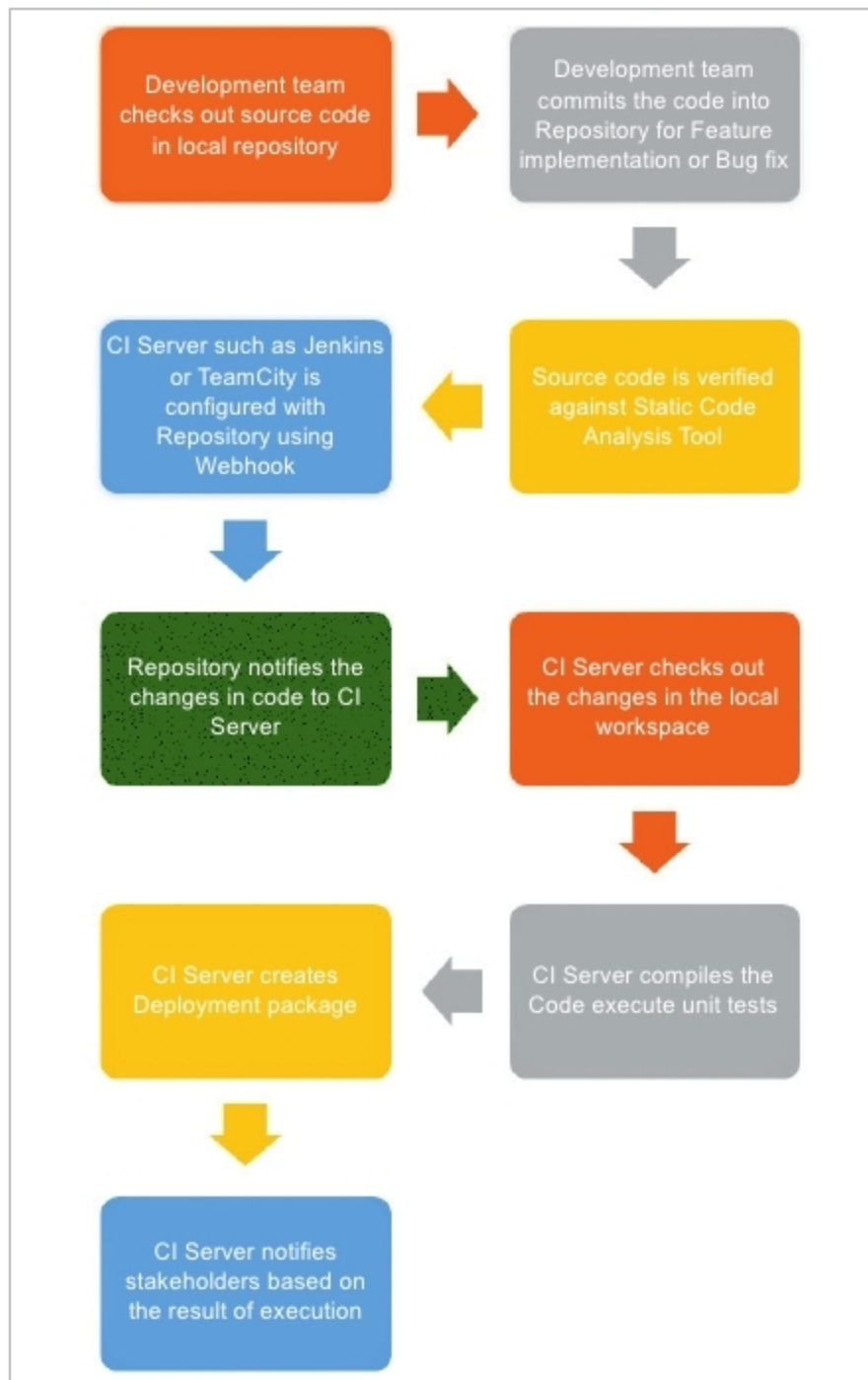
Figure 5: CI flow
