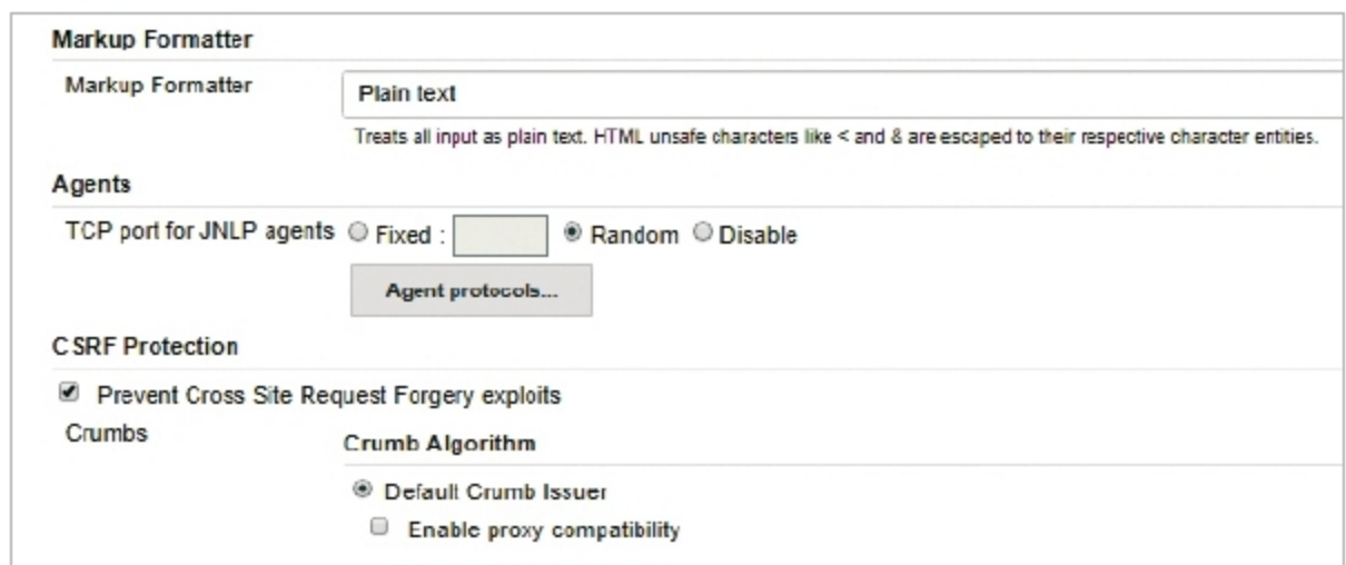
Figure 6: Agent protocol
