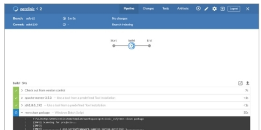
Figure 8: Blue Ocean - execution log
