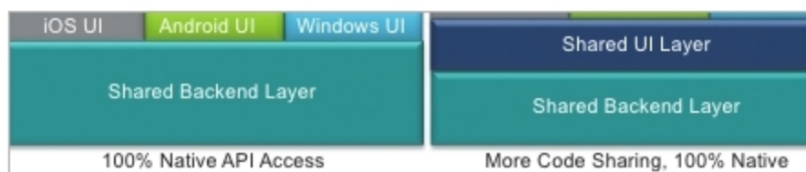
Figure 2: Xamarin Native and Xamarin Forms
