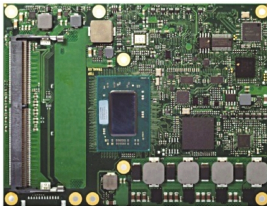
Figure 3: conga-TR4 with AMD Embedded Ryzen processor (Credit: congatec)
