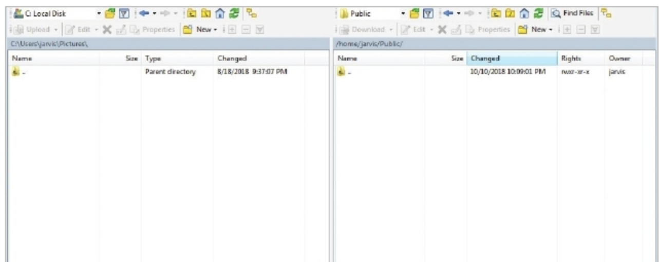
Figure 9: File sharing
