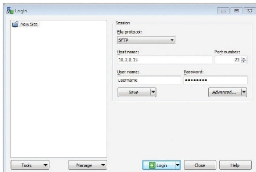
Figure 8: Connection settings
