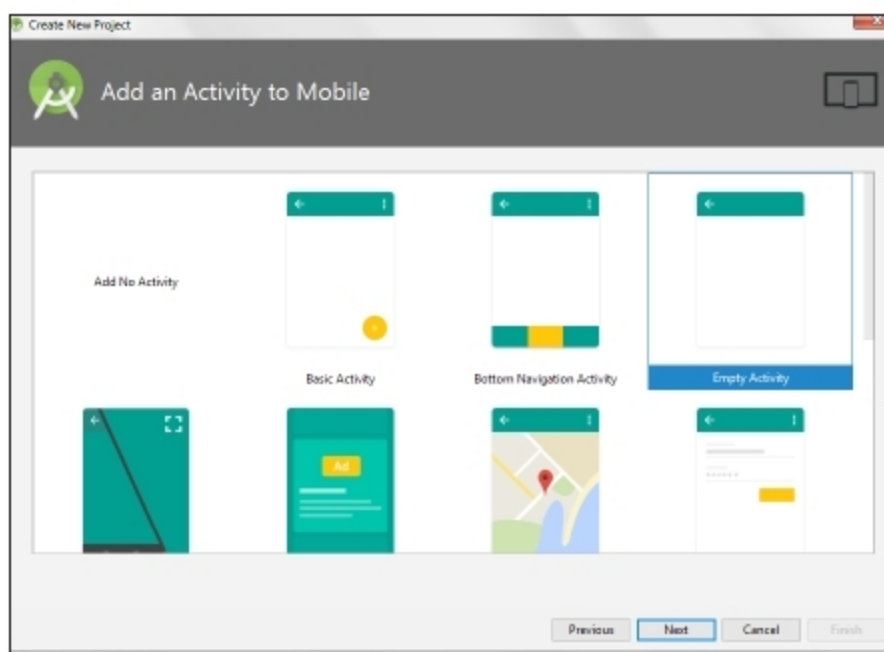
Figure 8: Activity
