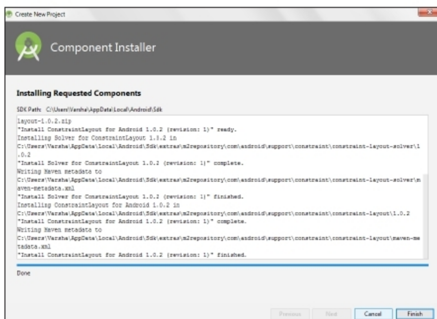
Figure 9: Component installer
