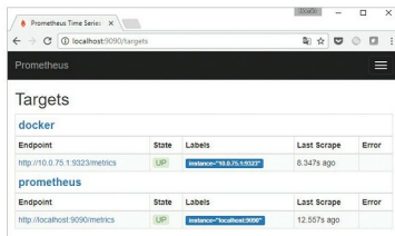
Figure 1: Prometheus targets
