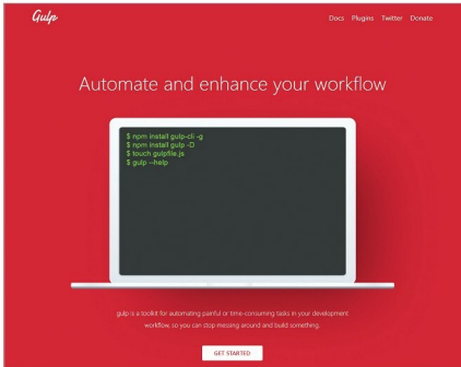
Figure 8: Gulp
