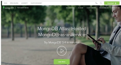
Figure 7: MongoDB
