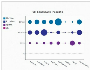
Figure 10: Pygal – Dot chart
