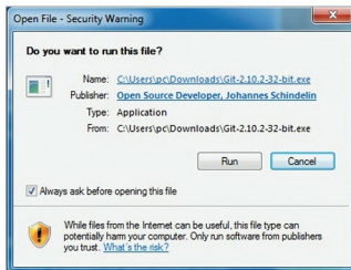
Figure 5: Installing Git
