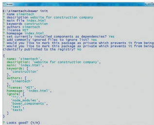
Figure 2: Creating bower.json
