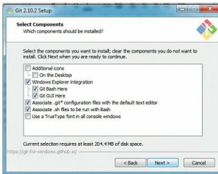
Figure 6: Selecting components
