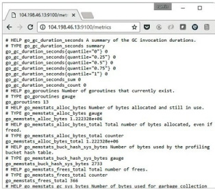
Figure 3: Node metrics
