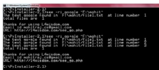
Figure 10: The power of regular expressions
