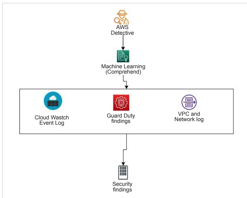
Figure 1: Amazon Detective
