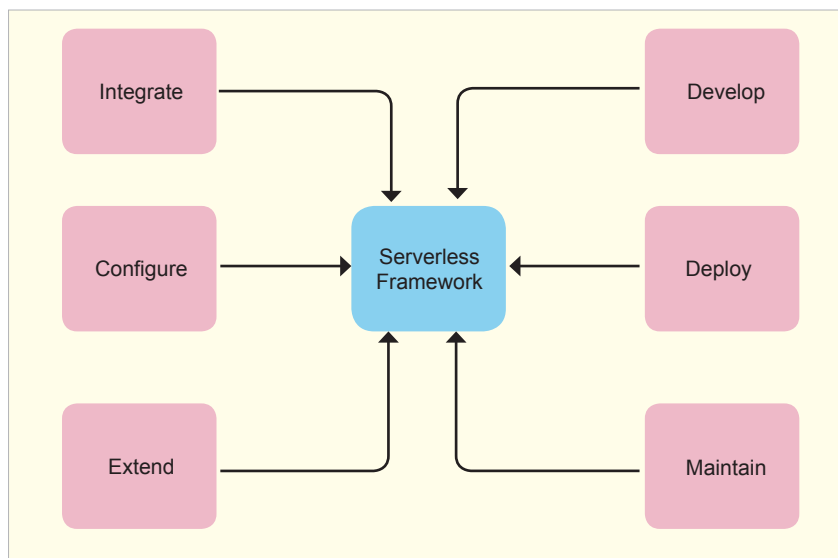
Figure 1: Serverless framework
