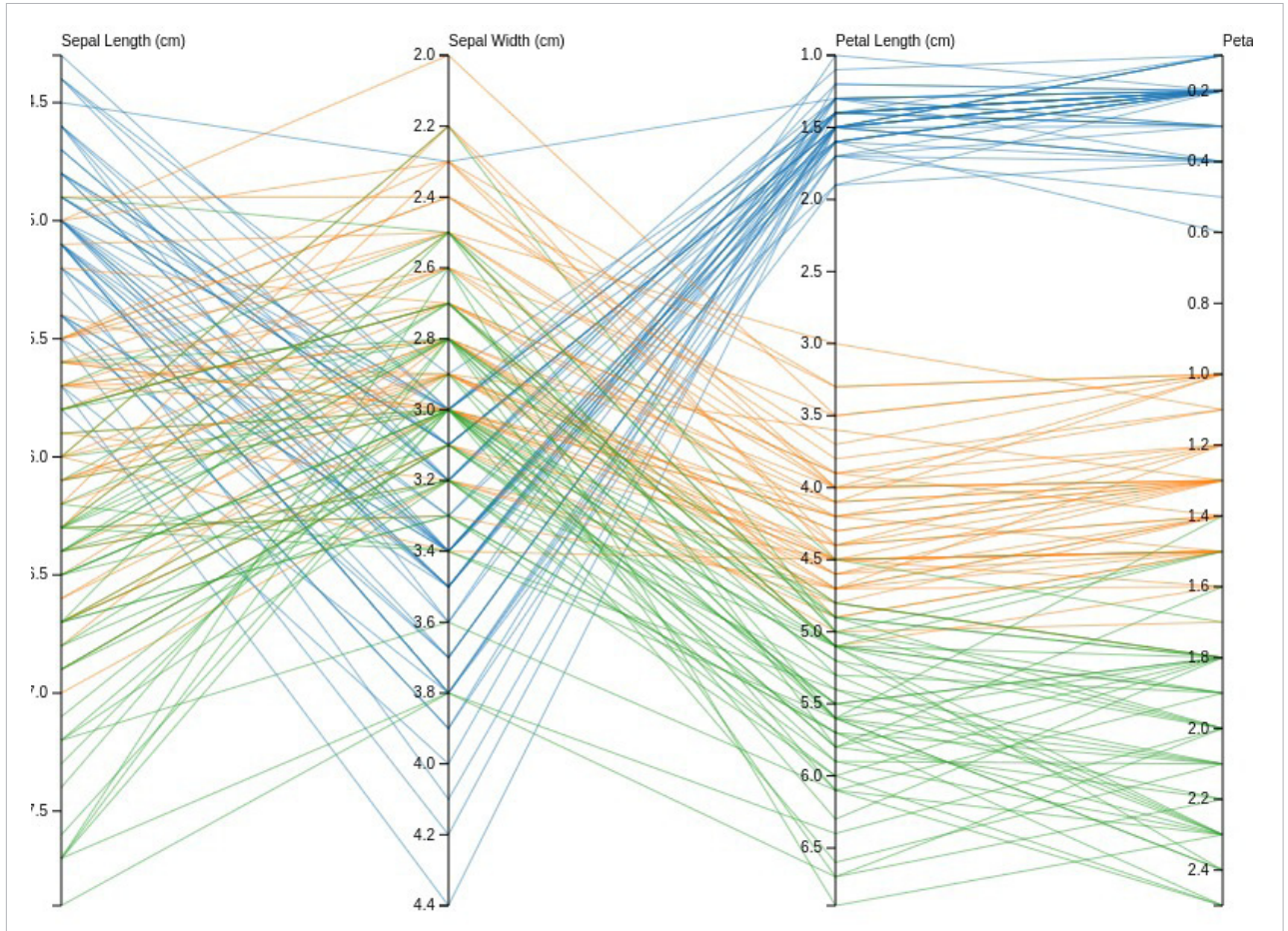
Figure 9: Parallel Coordinates Chart
